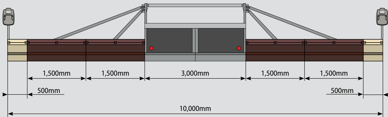
Example: SB 250 in TV or TP1 versions built up to maximum pave width
