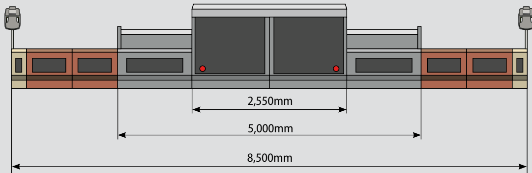
Example: AB 500 in TV or TP1 versions built up to maximum pave width
