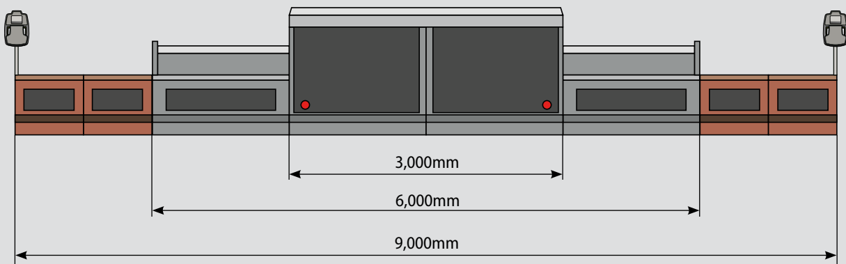
Example: AB 600 in TV or TP1 versions built up to maximum pave width
