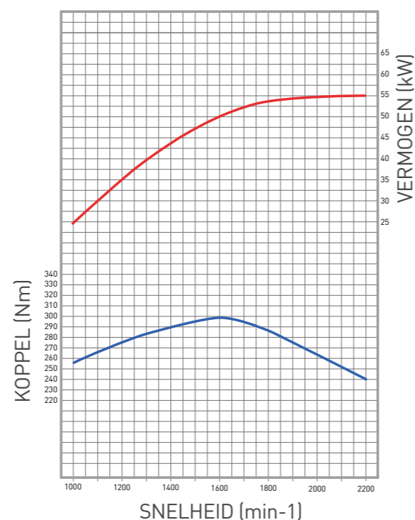
TCD 2.9 L4 MOTOR
