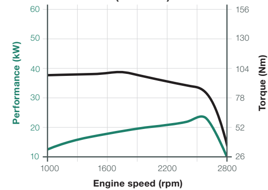
Performance curve of Yanmar 3TNV88; 24.1 kW; stage IIIA (standard)
