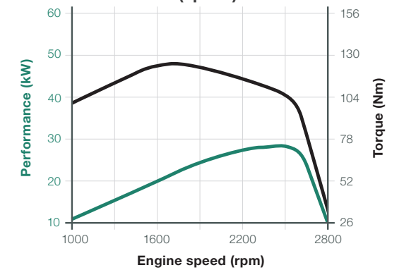
Performance curve of Yanmar 3TNV84; 26.7 kW; stage IIIA (option)
