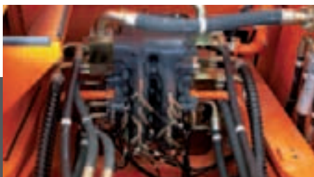
Control valve • Spool diameter : 35 mm • Main relief pressure: 320/350 bar
